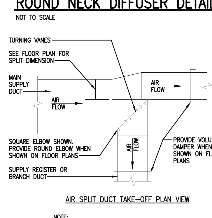
TYPICAL DIFFUSER RUNOUT DETAIL NOT TO SCALE
