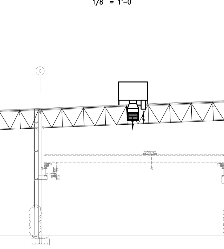
HVAC SECTION - PACKAGING AND SHIPPING AREA 1/8" = 1'-0"
