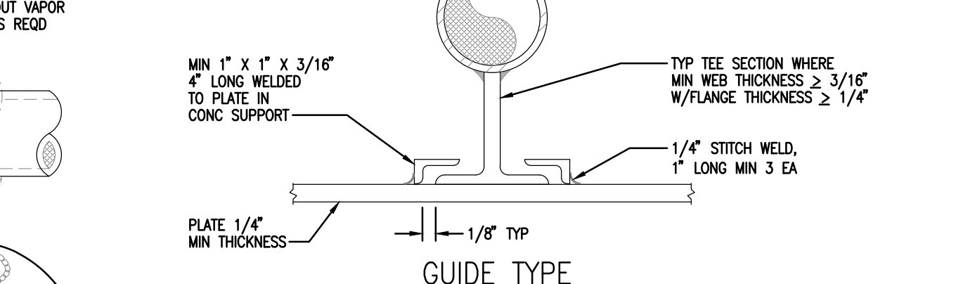
GRID HORIZONTAL MOUNTING DETAIL FOR CW PIPES 4" TO 8" PIPE INSIDE BUILDING NOT TO SCALE
