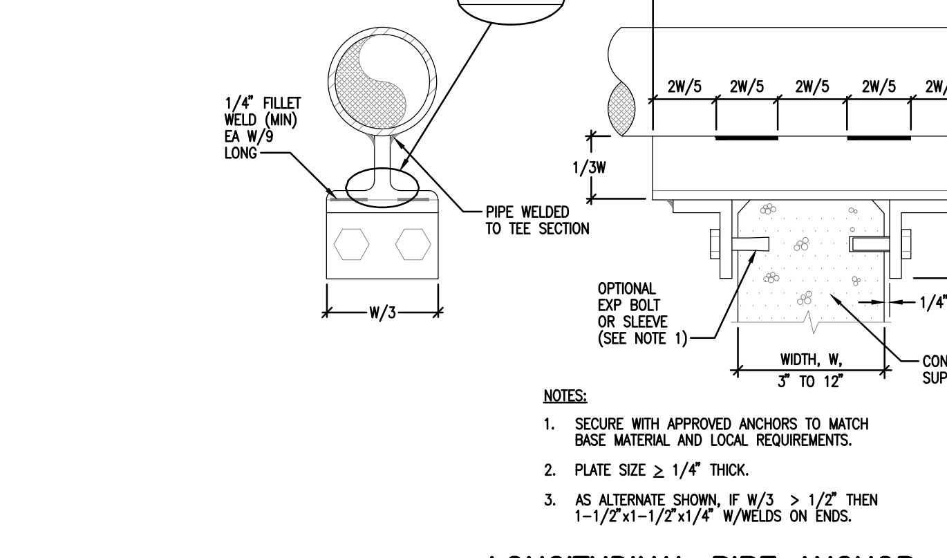
LONGITUDINAL PIPE ANCHOR NOT TO SCALE
