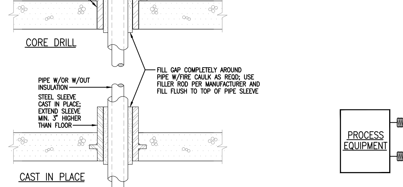
LONGITUDINAL PIPE ANCHOR NOT TO SCALE
