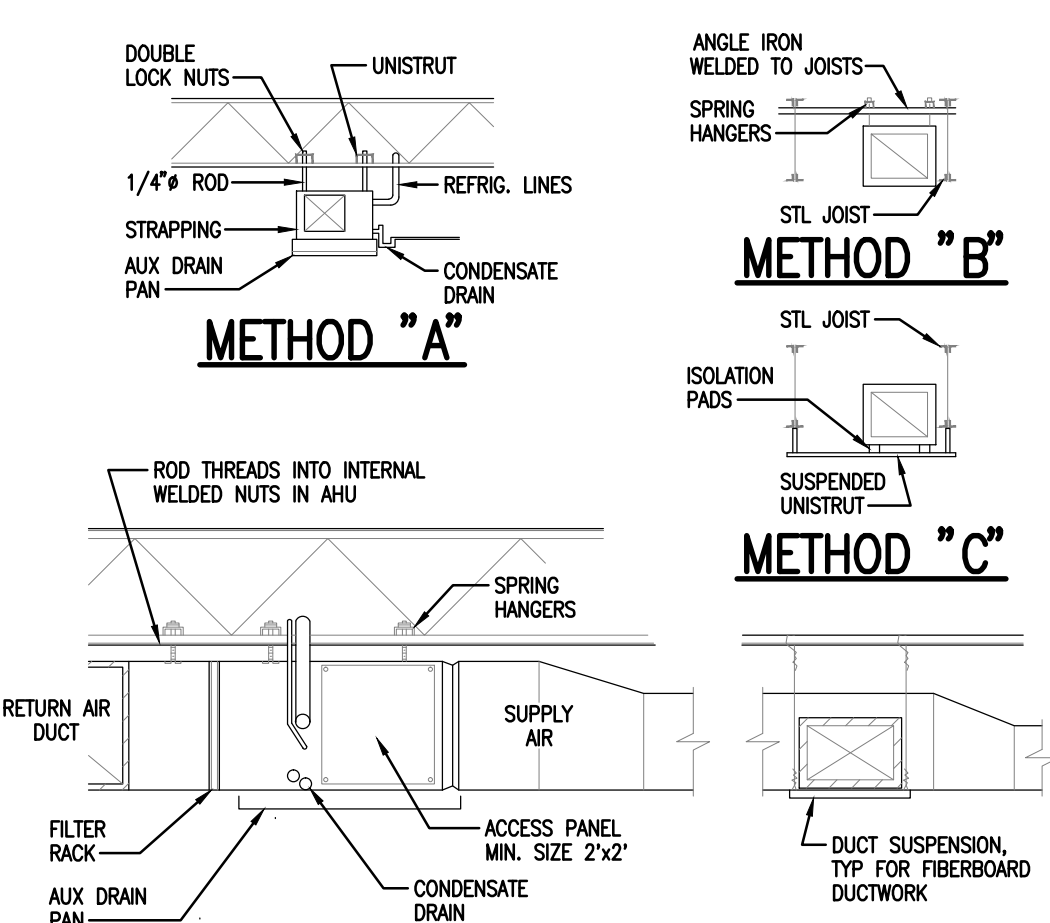
ABOVE CEILING AHU SUSPENSION ARRANGEMENT NOT TO SCALE
