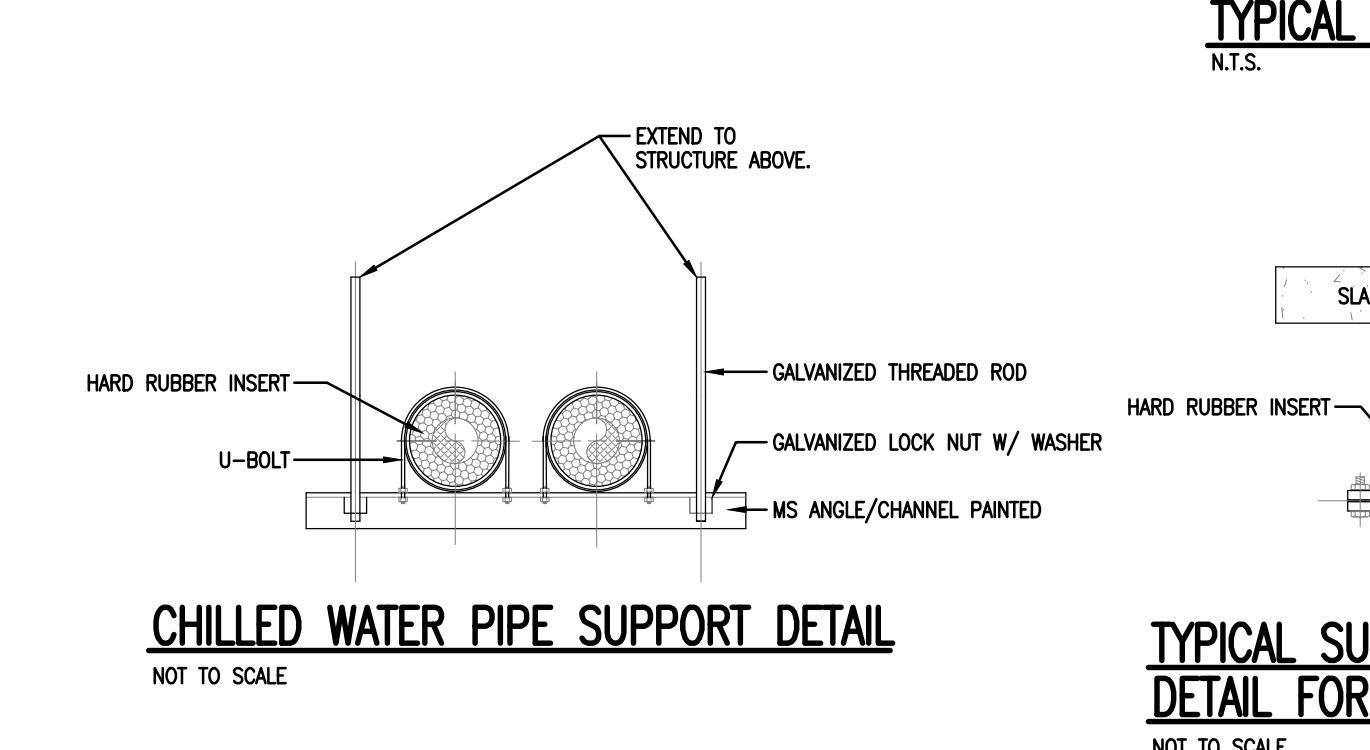
TYPICAL SUSPENSION FROM SLAB DETAIL FOR CW PIPES UP TO 2" NOT TO SCALE
