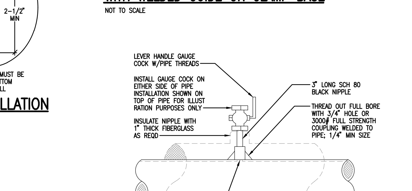
PIPE IN TRENCH DETAIL NOT TO SCALE
