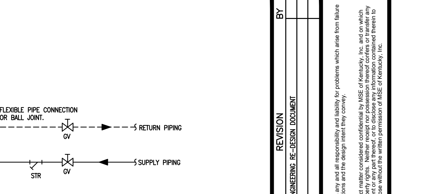
TYPICAL PROCESS EQUIPMENT CONNECTION DETAIL NOT TO SCALE
