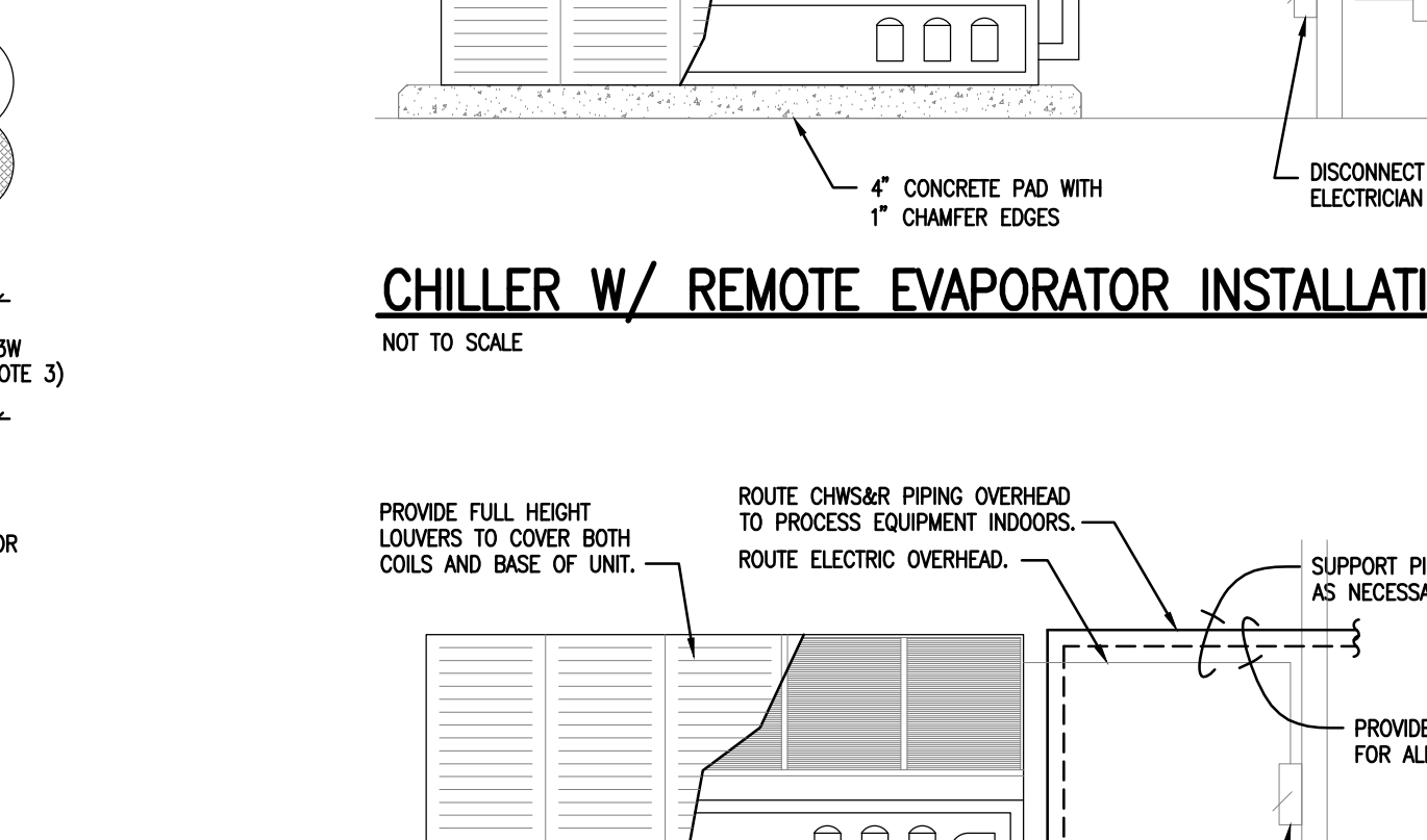
PACKAGED CHILLER INSTALLATION DETAIL NOT TO SCALE
