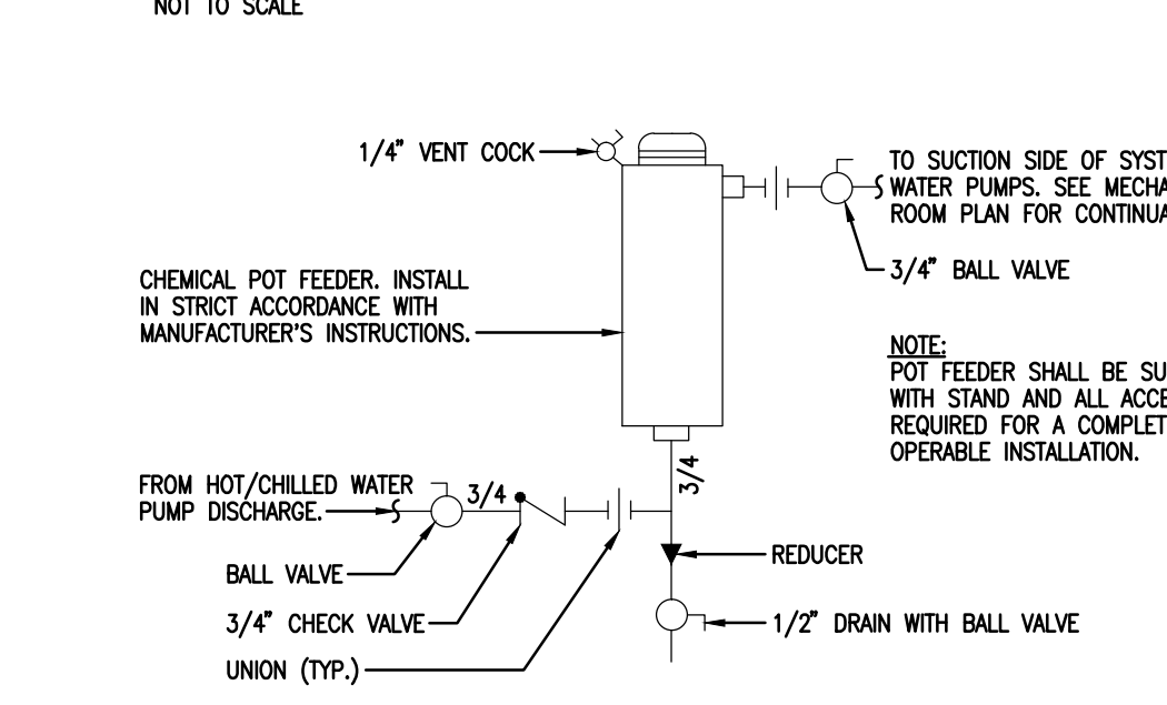
POT FEEDER PIPING DETAIL NOT TO SCALE
