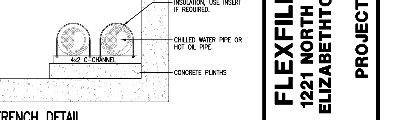
PIPE IN TRENCH DETAIL NOT TO SCALE
