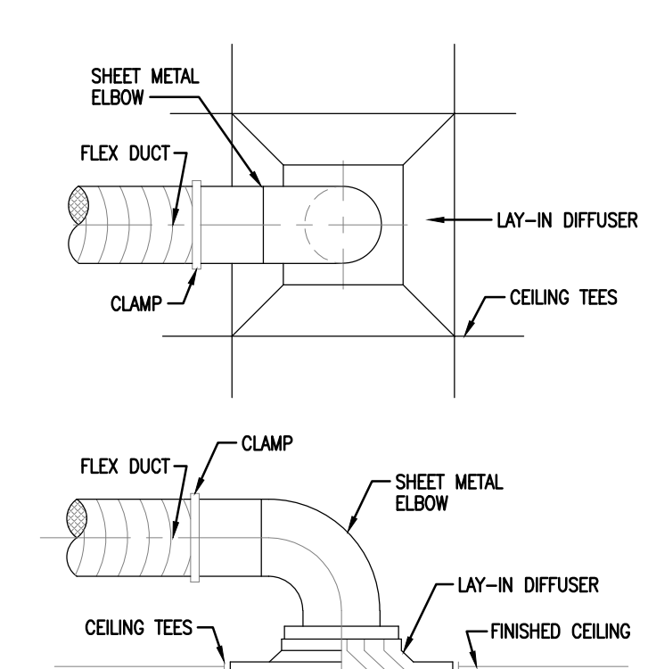
ROUND NECK DIFFUSER DETAIL NOT TO SCALE
