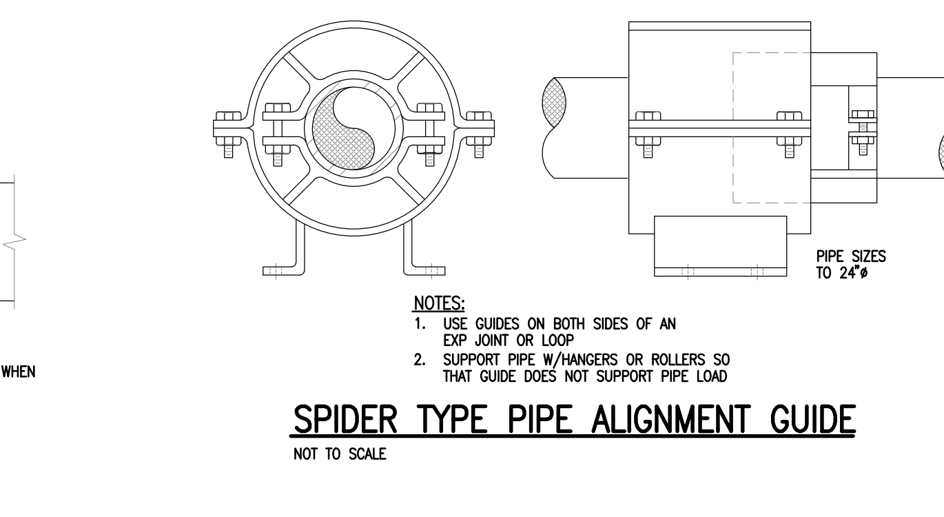
CHILLED WATER PIPE SUPPORT DETAIL NOT TO SCALE
