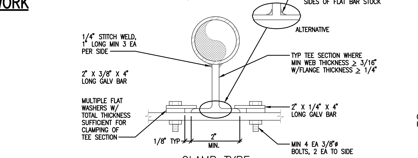
TYPICAL SUSPENSION FROM SLAB DETAIL FOR CW PIPES UP TO 2" NOT TO SCALE
