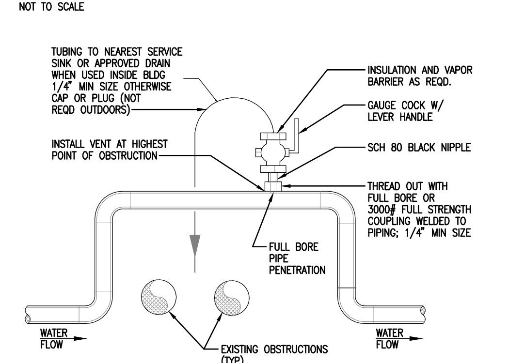
HIGH POINT MANUAL AIR VENT NOT TO SCALE
