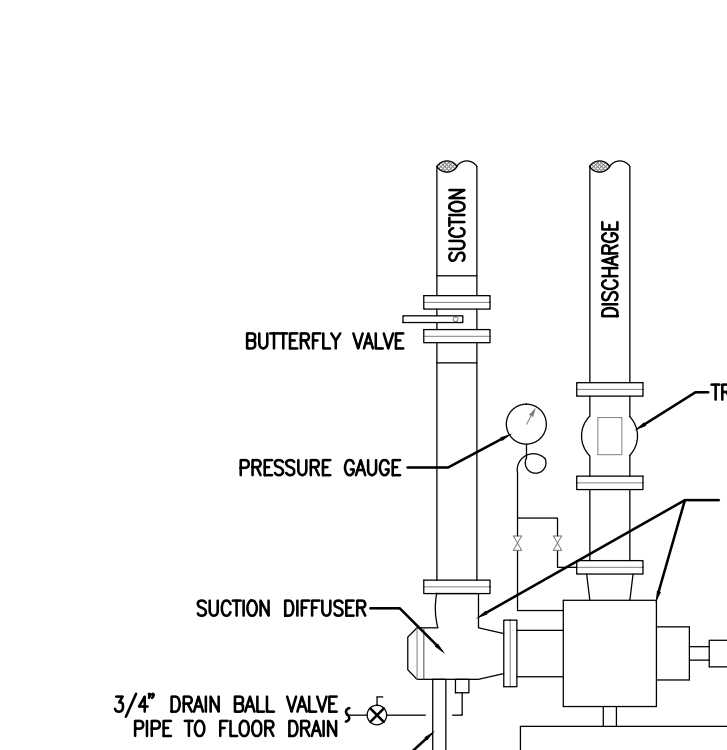
TYPICAL BASE MOUNTED PUMP SCHEMATIC NOT TO SCALE
